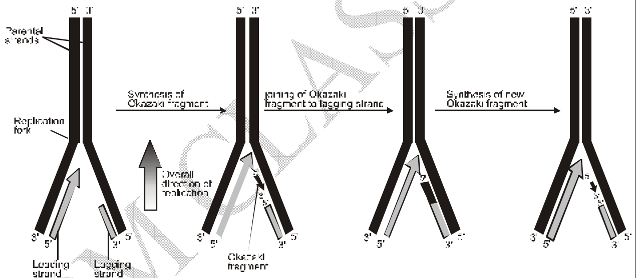
Figure : Synthesis of leading and lagging strands of DNA. The leading strand is synthesized continuously in the direction of replication fork movement. The lagging strand is synthesized in small pieces (Okazaki fragments) backward from the overall direction of replication. The Okazaki fragments are then joined by the action of DNA ligase.
