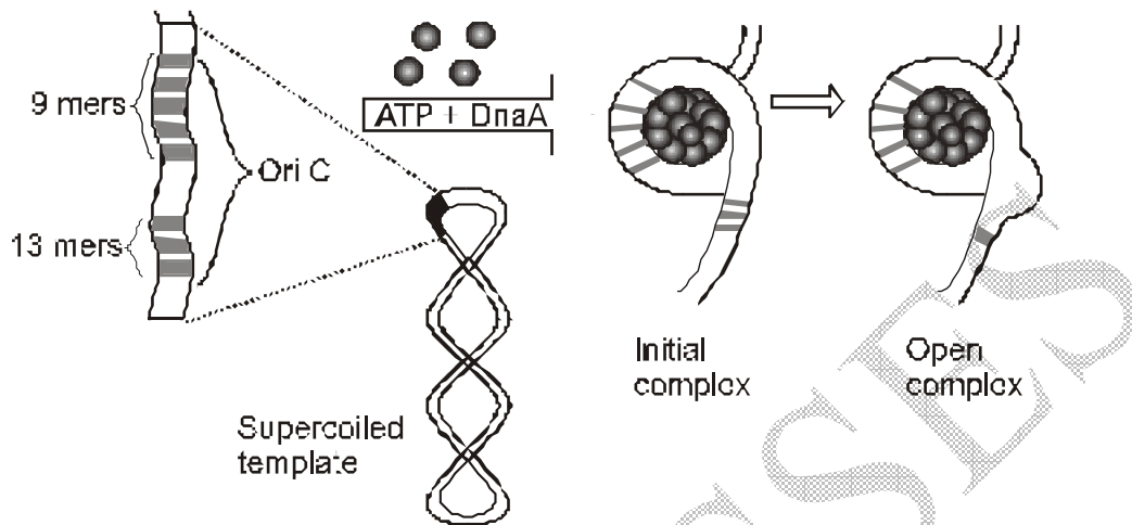
Fig. Initiation at oriC occurs after DnaA protein binds the five 9 mers. The 13 mer region is then denatured, and this open complex serves as a replication start site.
