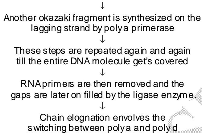
Fig. 4 Process of Eukaryotic Replication
