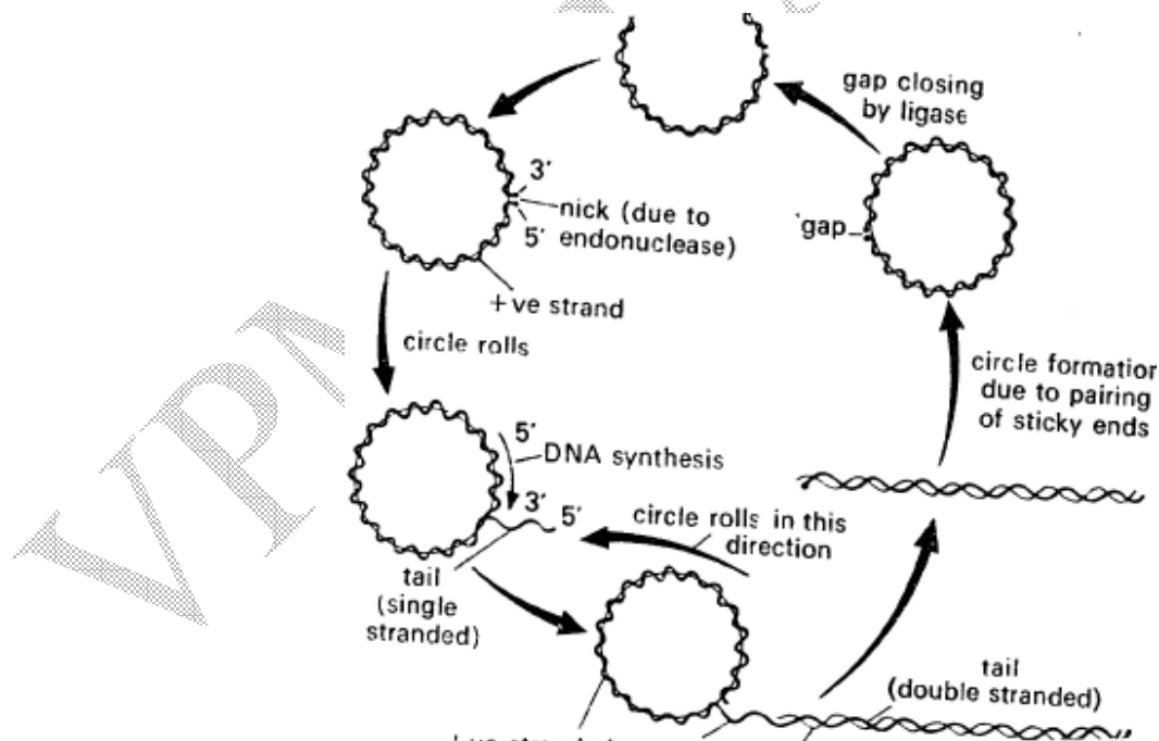
FIG: 6 ROLLING CIRCLE MODEL OF DNA REPLICATION
