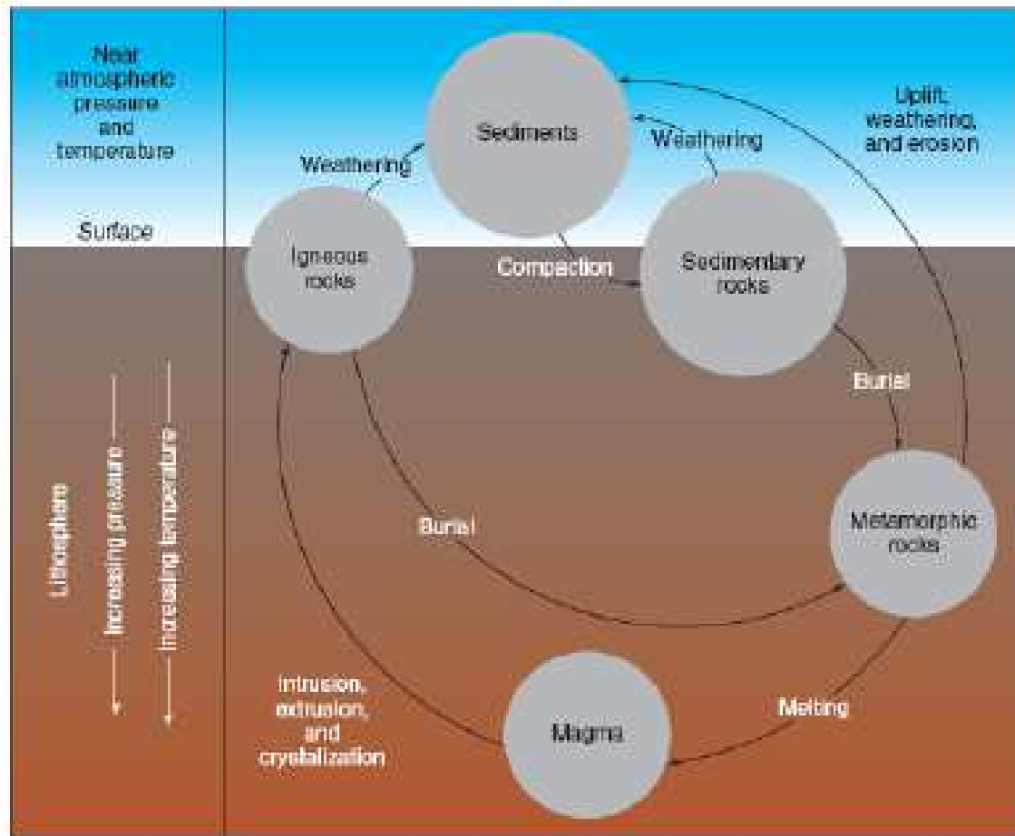
Fig.4 Rock Cycle
