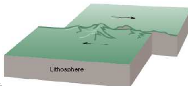
FIG :7 A transform plate boundary is often the site of shallow earthquakes
